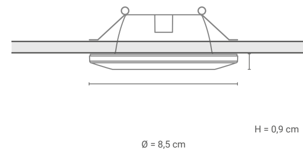
thevios 3 for flush mounting
