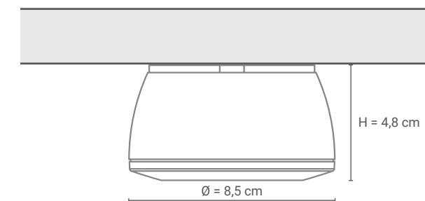
thevios 3 for surface mounting
