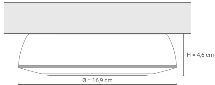
thevios 5 for surface mounting
